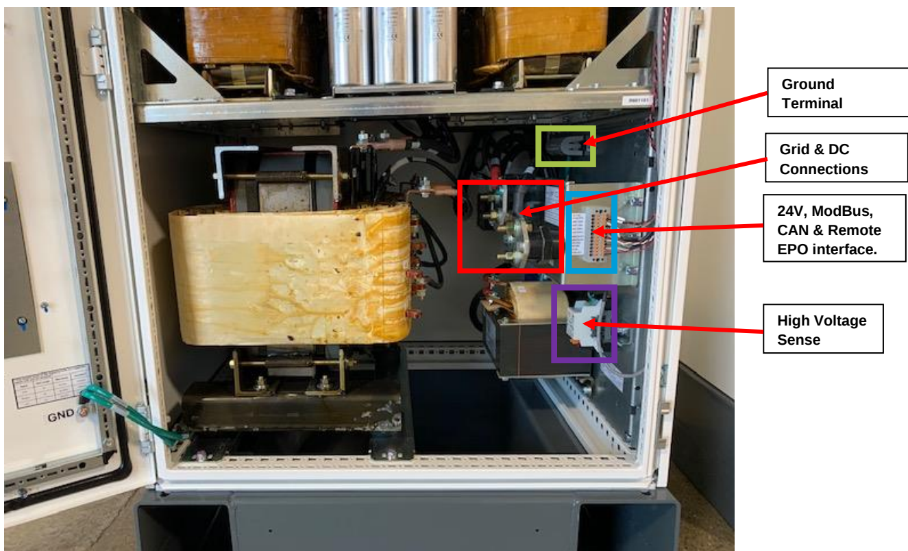
GRID & DC CONNECTIONS LOCATED VIEW
