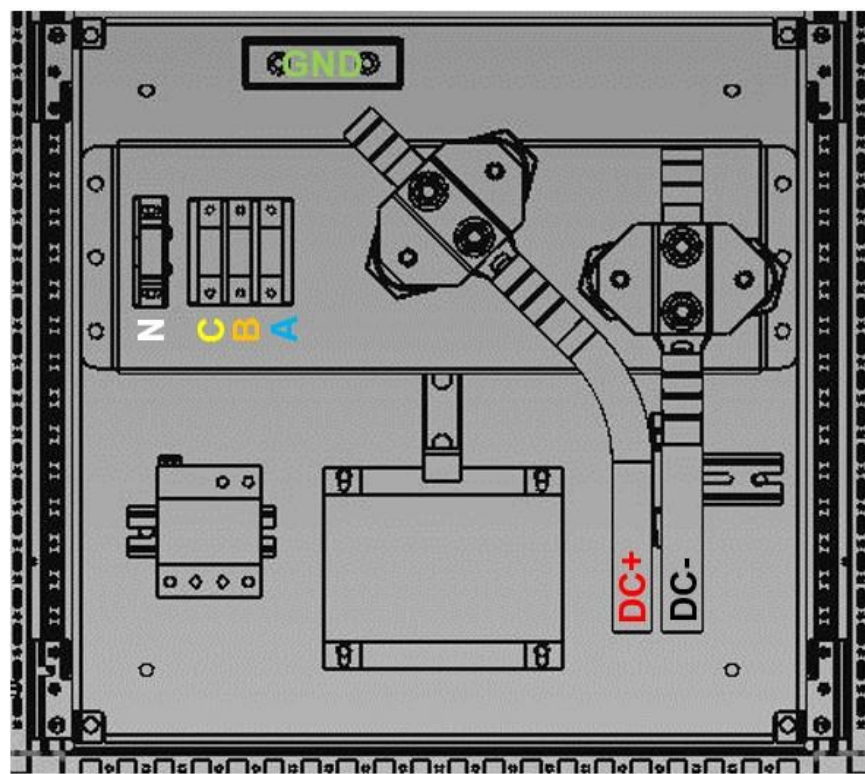
RIGHT-SIDE PANEL VIEW (DC+, DC-, GND)
